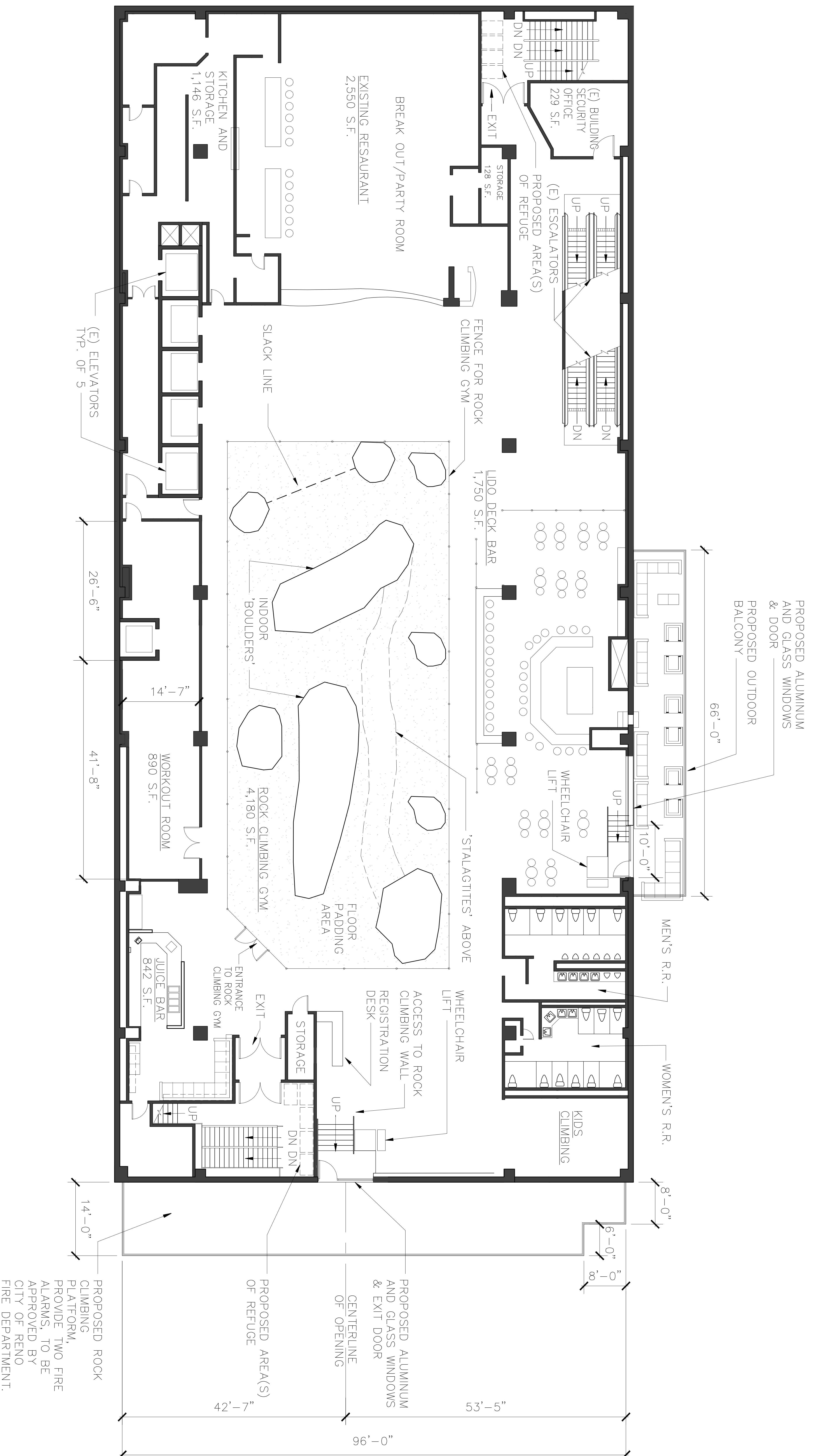
1 PROPOSED SECOND FLOOR PLAN SCALE: 1/8" = 1'-0" NORTH
